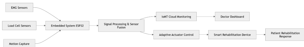
Figure 2. IoMT Rehabilitation System Architecture Diagram
